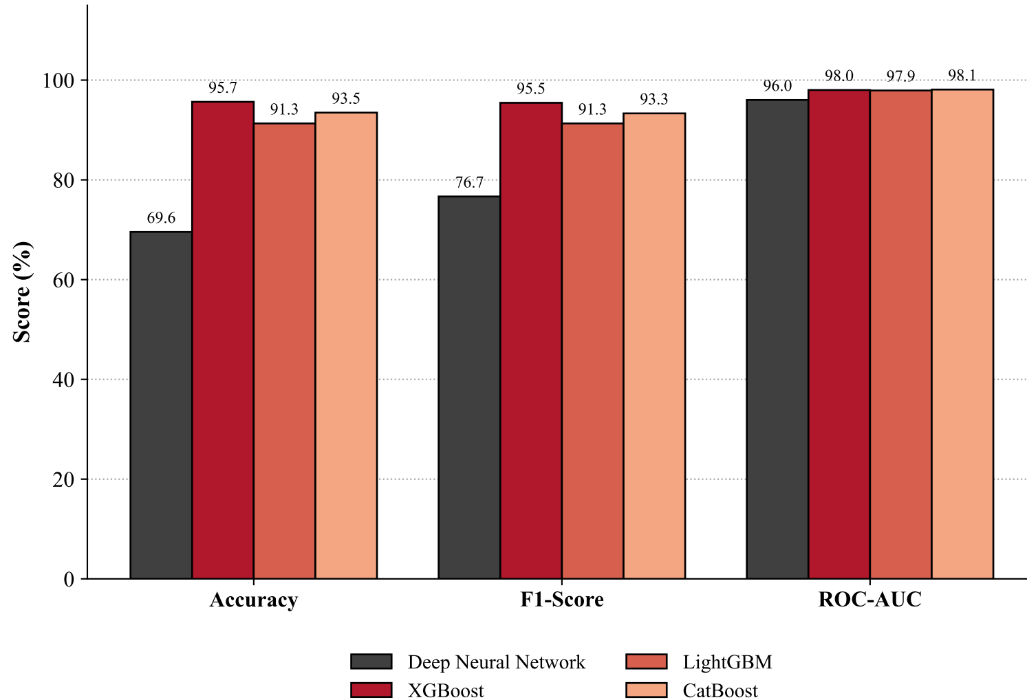
A: Metric Comparison on High-Dimensional Tabular Data
