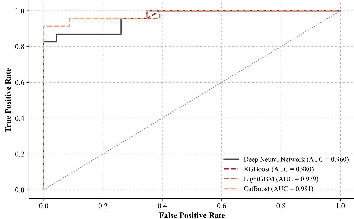
B: ROC Curve Analysis
